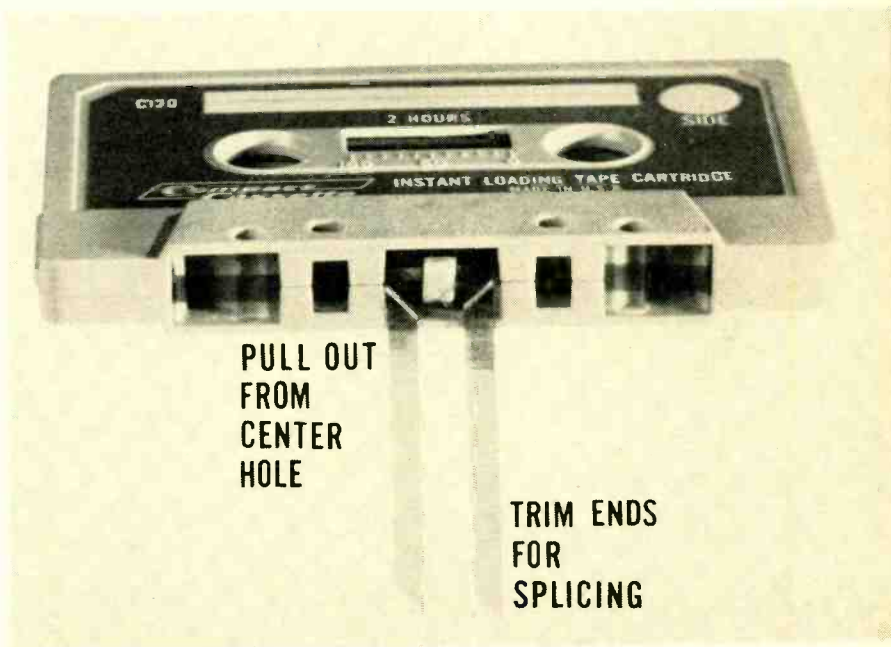
FIG. 3—TO TRANSFER TAPE from jammed cassette to new cassette, start by pulling out and cutting tape leader end. See text for full description.
